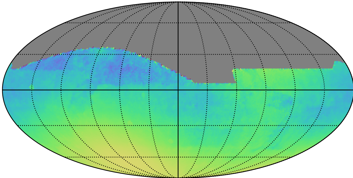
mw_roll_all_v3.3_10yrs All sky: Normalized Parallax Uncert @ 22.4
