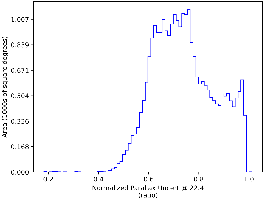
mw_roll_all_v3.3_10yrs All sky: Normalized Parallax Uncert @ 22.4
