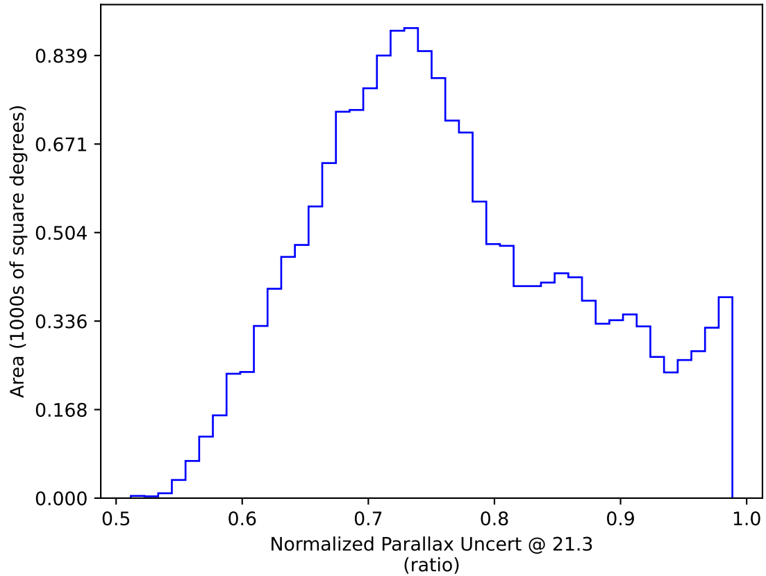
mw_roll_all_v3.3_10yrs WFD y band only: Normalized Parallax Uncert @ 21.3
