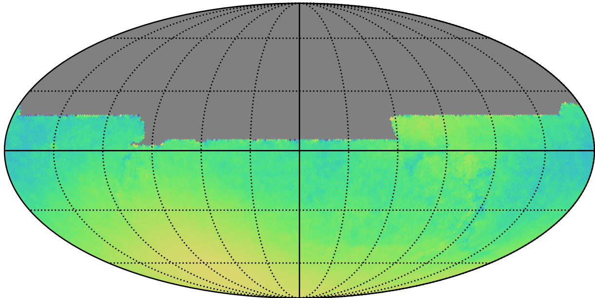
mw_roll_all_v3.3_10yrs All sky y band only: Normalized Parallax Uncert @ 21.3
