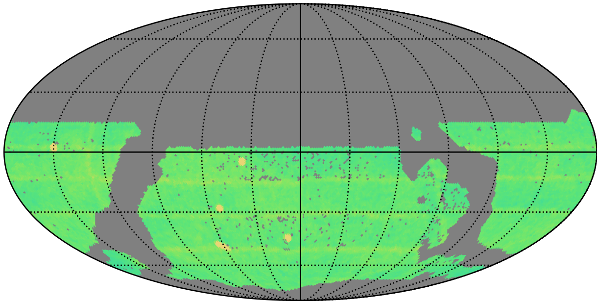
mw_roll_all_v3.3_10yrs WFD all bands: N Unique Nights
