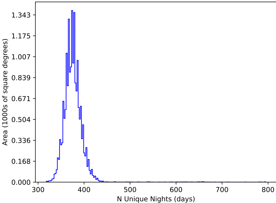
mw_roll_all_v3.3_10yrs WFD all bands: N Unique Nights
