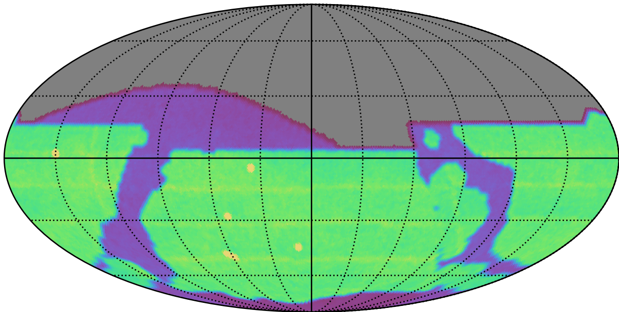
mw_roll_all_v3.3_10yrs All sky all bands: N Unique Nights
