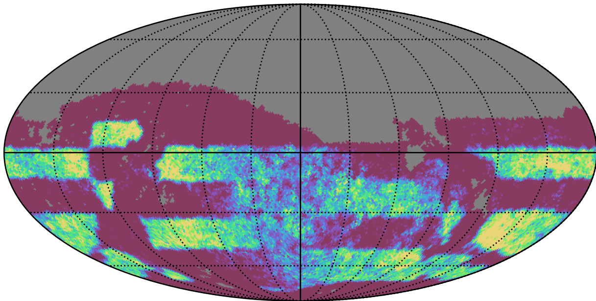
mw_roll_all_v3.3_10yrs Yr 3-4 z band: NVisits
