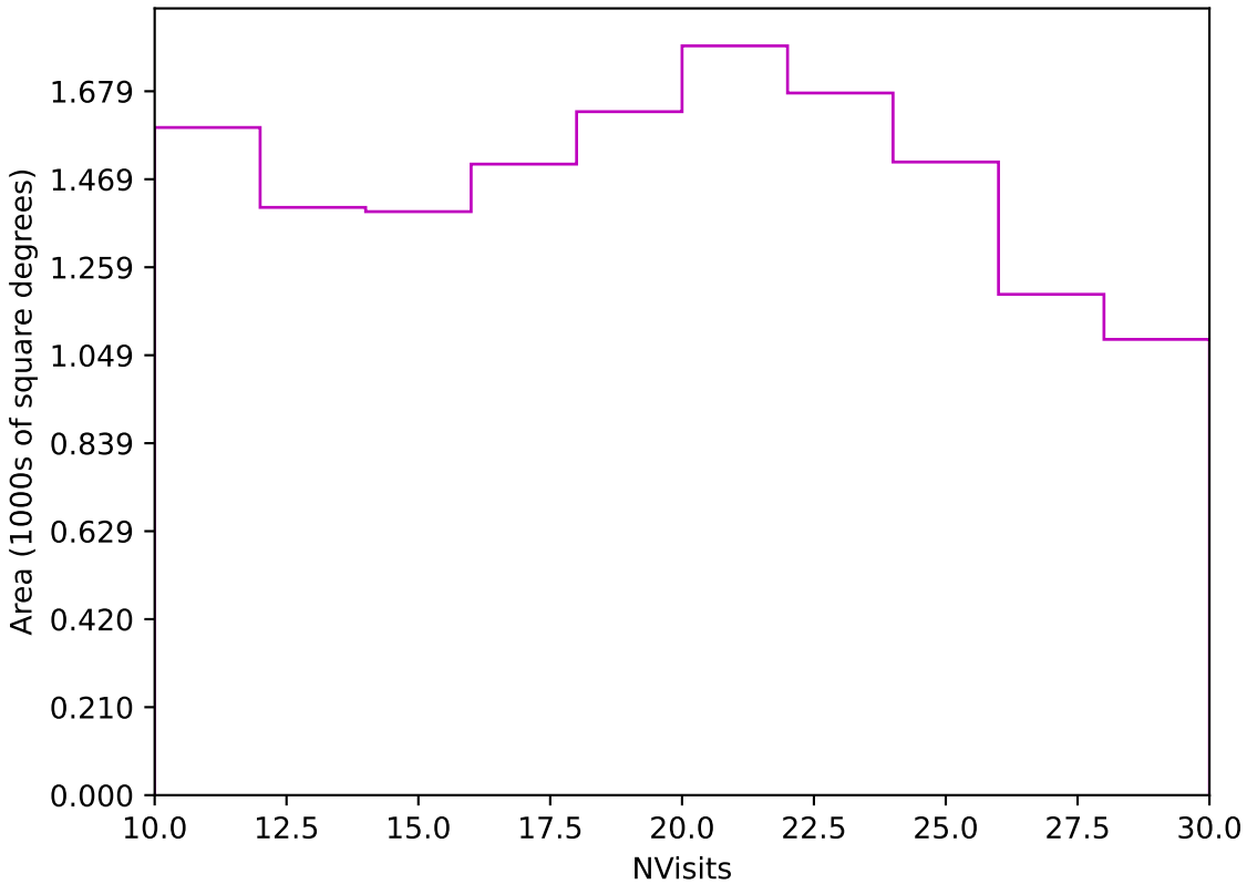
mw_roll_all_v3.3_10yrs Yr 3-4 z band: NVisits
