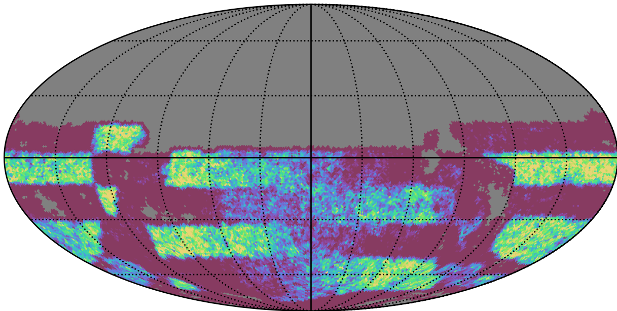
mw_roll_all_v3.3_10yrs Yr 3-4 y band: NVisits
