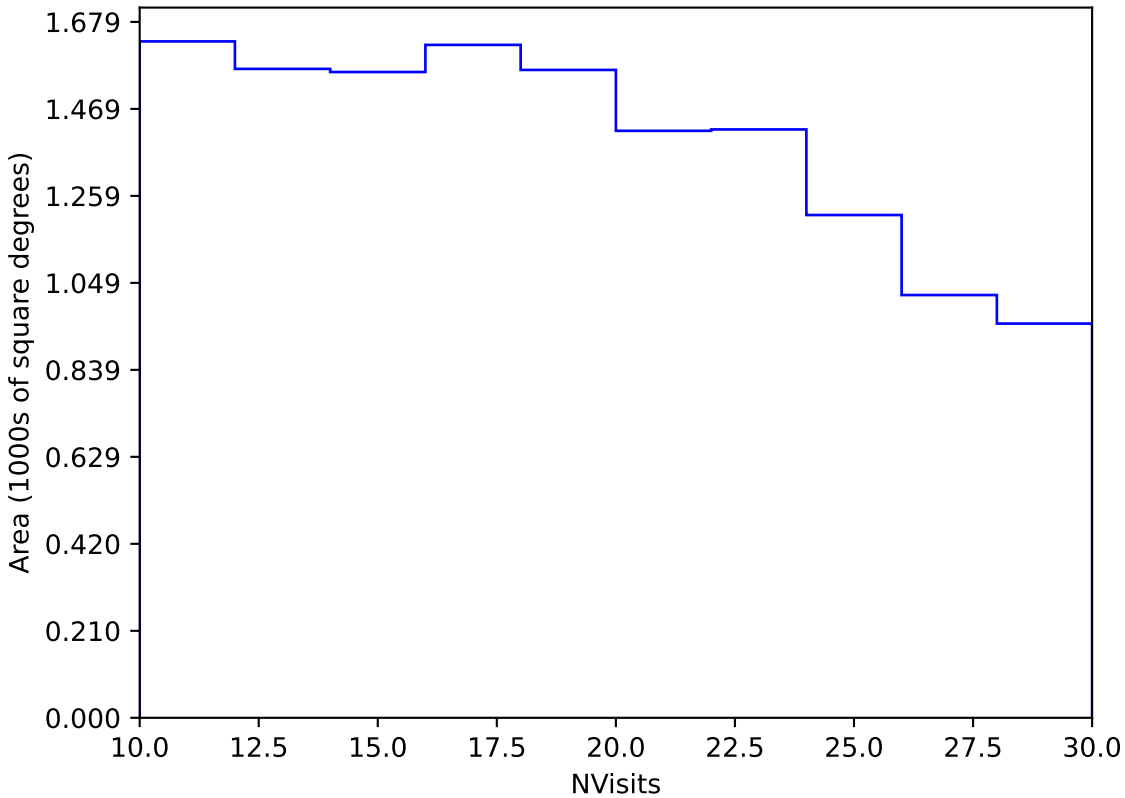
mw_roll_all_v3.3_10yrs Yr 3-4 y band: NVisits
