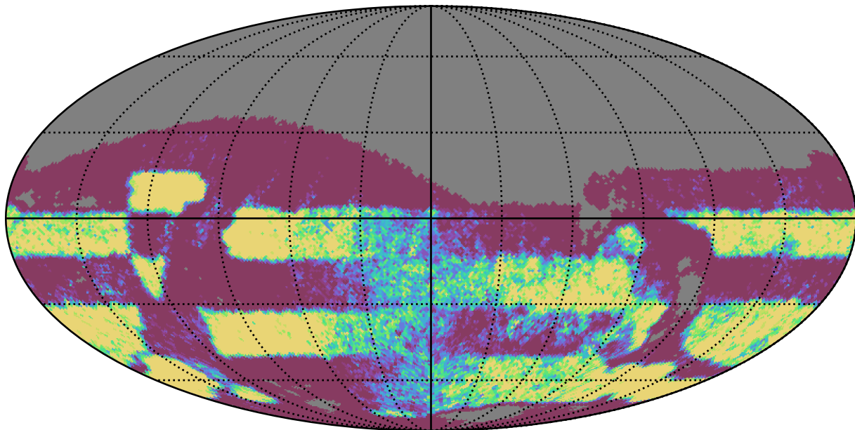
mw_roll_all_v3.3_10yrs Yr 3-4 r band: NVisits
