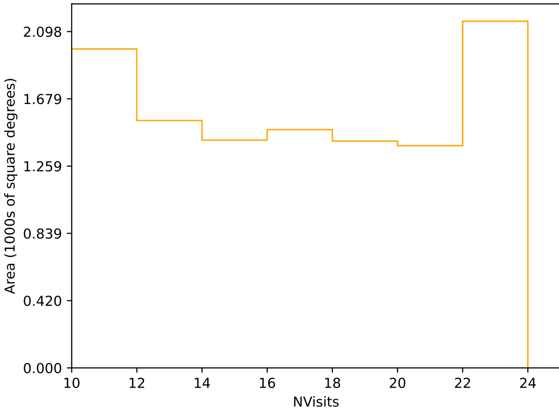
mw_roll_all_v3.3_10yrs Yr 3-4 r band: NVisits
