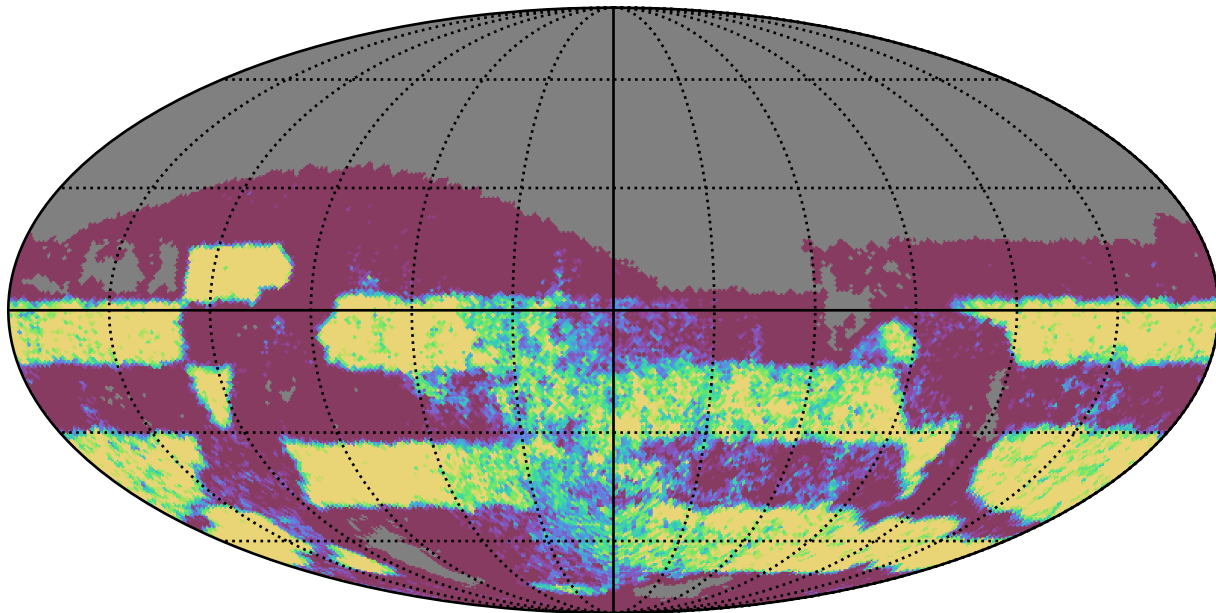
mw_roll_all_v3.3_10yrs Yr 3-4 i band: NVisits
