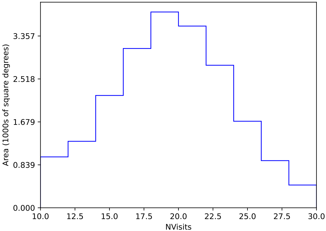
mw_roll_all_v3.3_10yrs Yr 1 y band: NVisits
