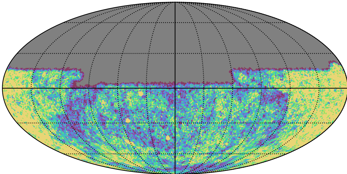
mw_roll_all_v3.3_10yrs Yr 1 u band: NVisits
