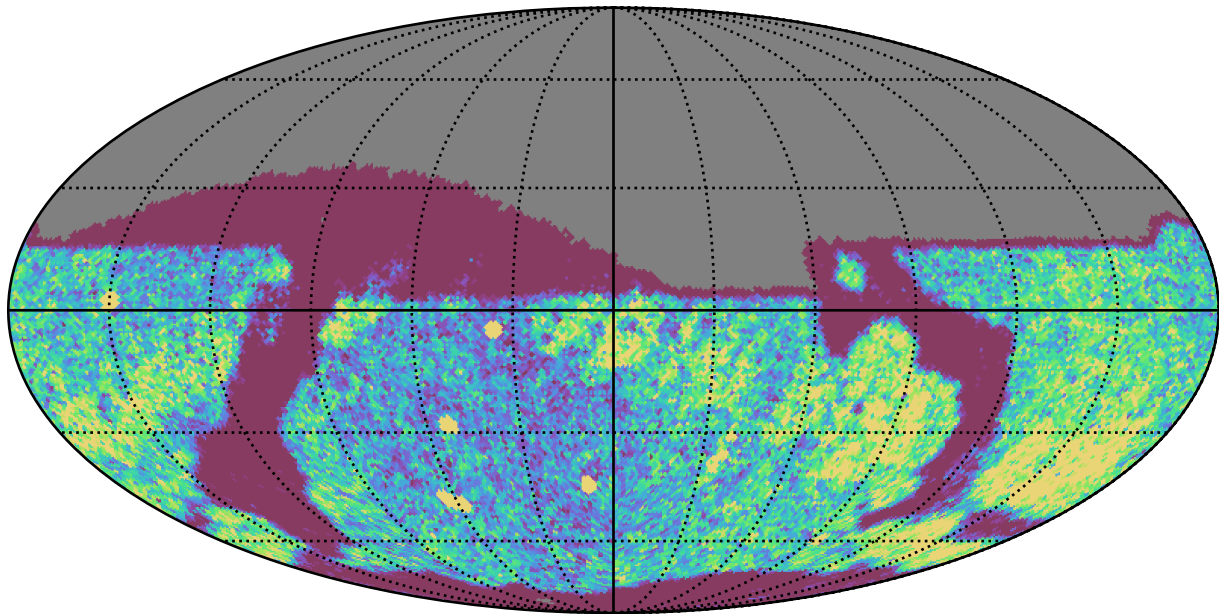
mw_roll_all_v3.3_10yrs Yr 1 r band: NVisits
