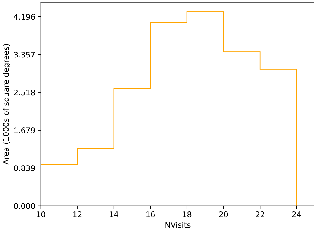
mw_roll_all_v3.3_10yrs Yr 1 r band: NVisits
