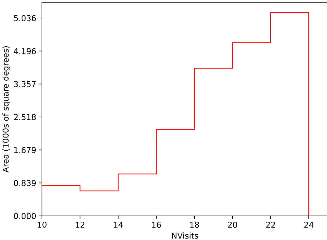
mw_roll_all_v3.3_10yrs Yr 1 i band: NVisits
