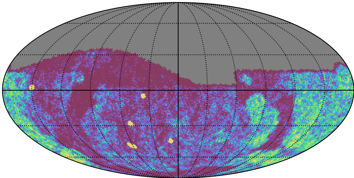
mw_roll_all_v3.3_10yrs Yr 1 g band: NVisits
