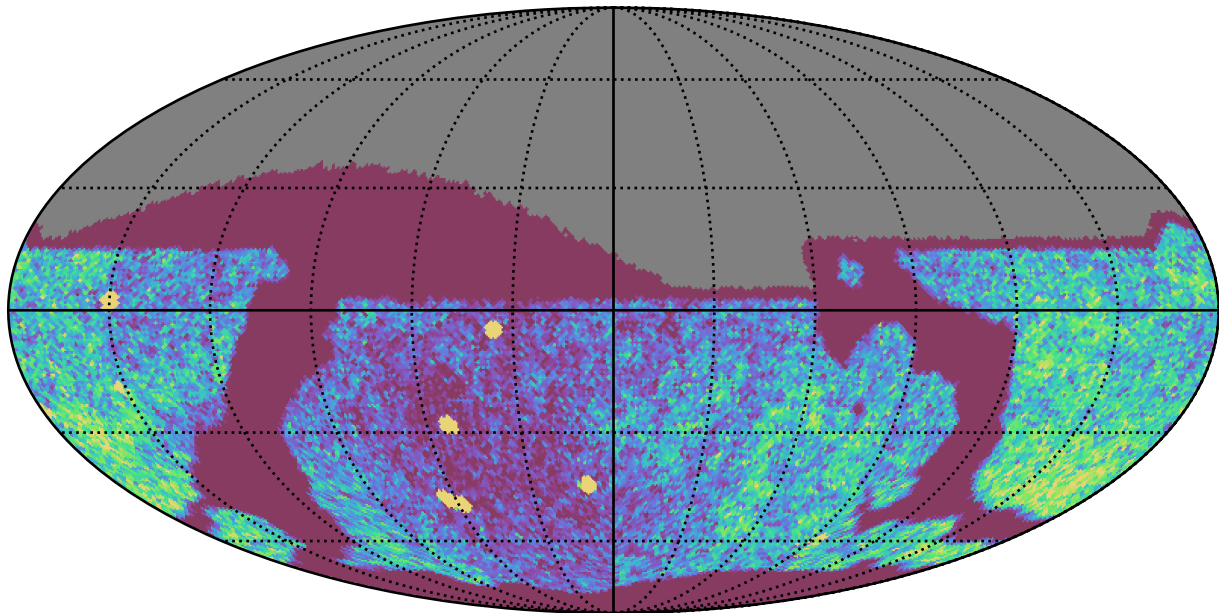
mw_roll_all_v3.3_10yrs Yr 1 all bands: NVisits
