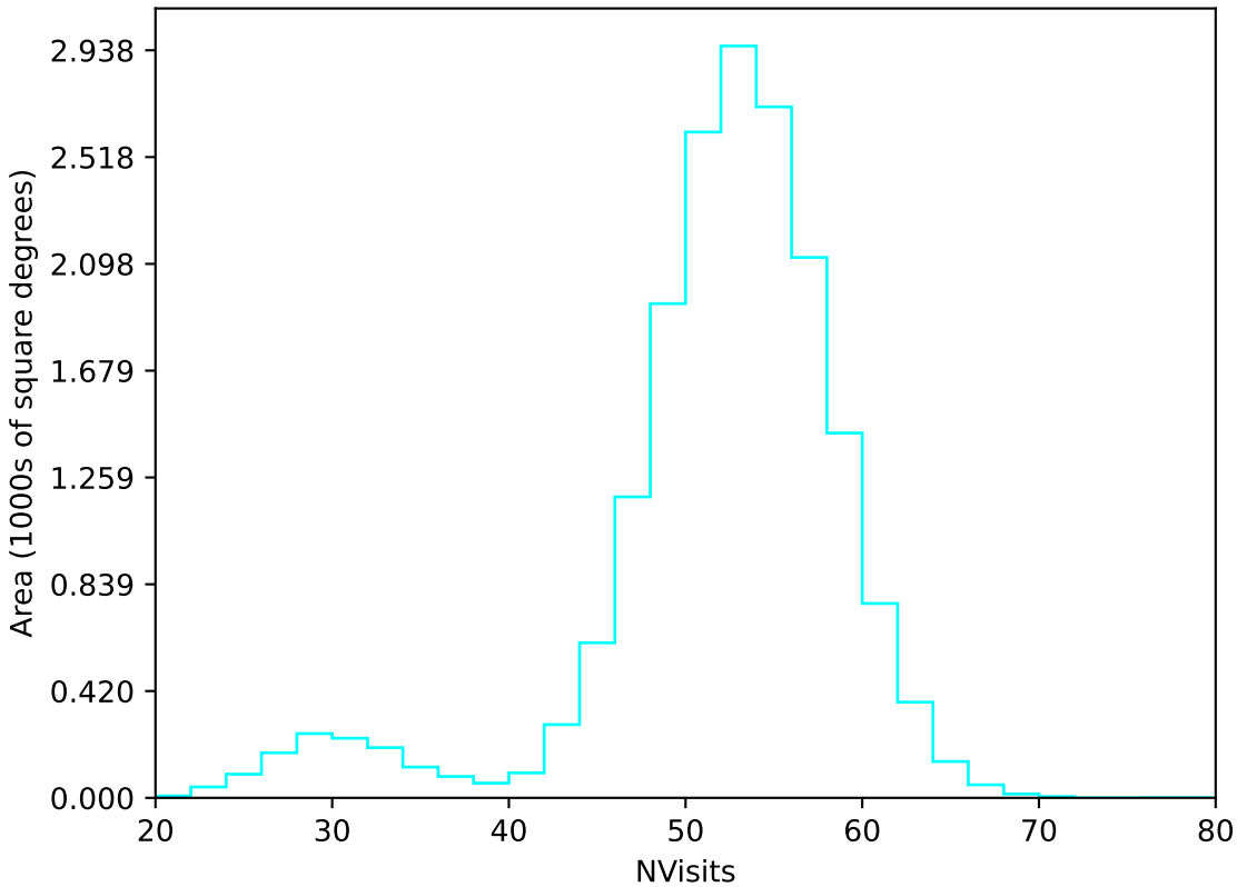
mw_roll_all_v3.3_10yrs WFD u band: NVisits
