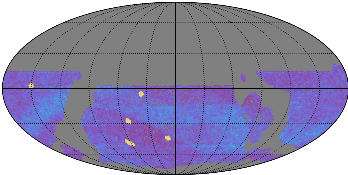
mw_roll_all_v3.3_10yrs WFD all bands: NVisits
