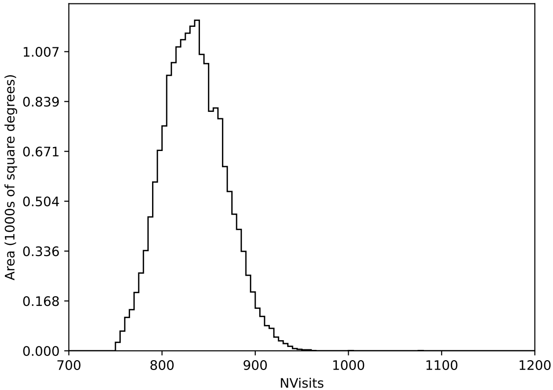
mw_roll_all_v3.3_10yrs WFD all bands: NVisits
