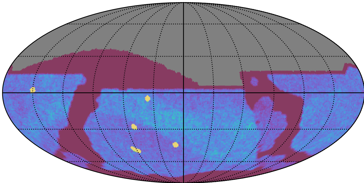
mw_roll_all_v3.3_10yrs All sky z band: NVisits
