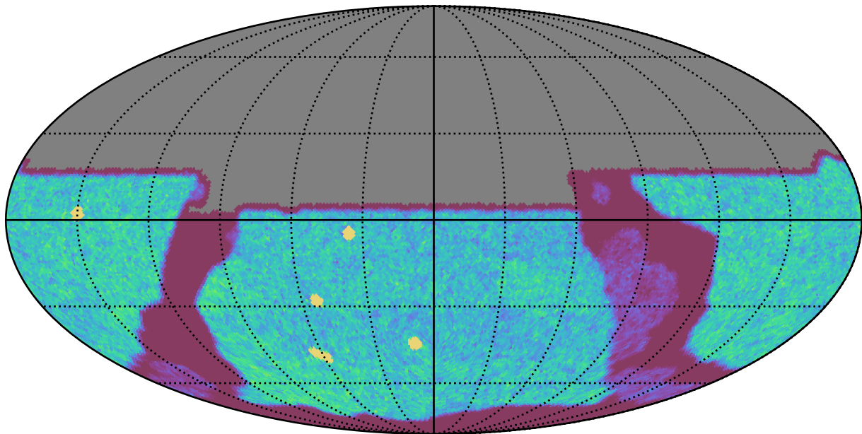
mw_roll_all_v3.3_10yrs All sky u band: NVisits
