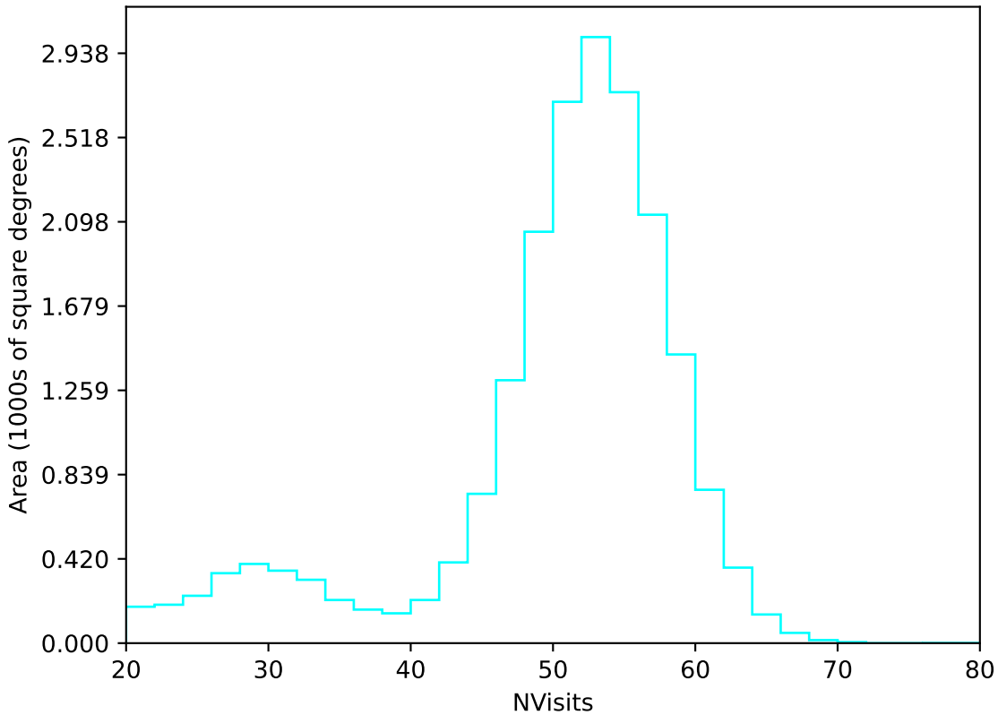
mw_roll_all_v3.3_10yrs All sky u band: NVisits
