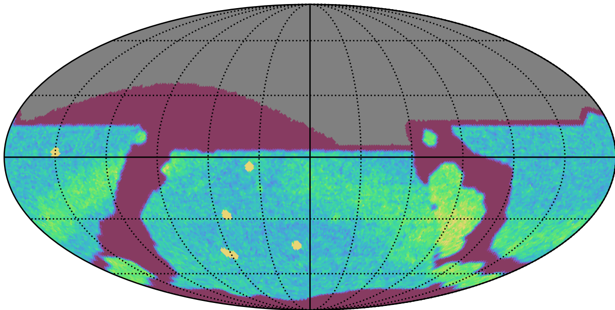
mw_roll_all_v3.3_10yrs All sky r band: NVisits
