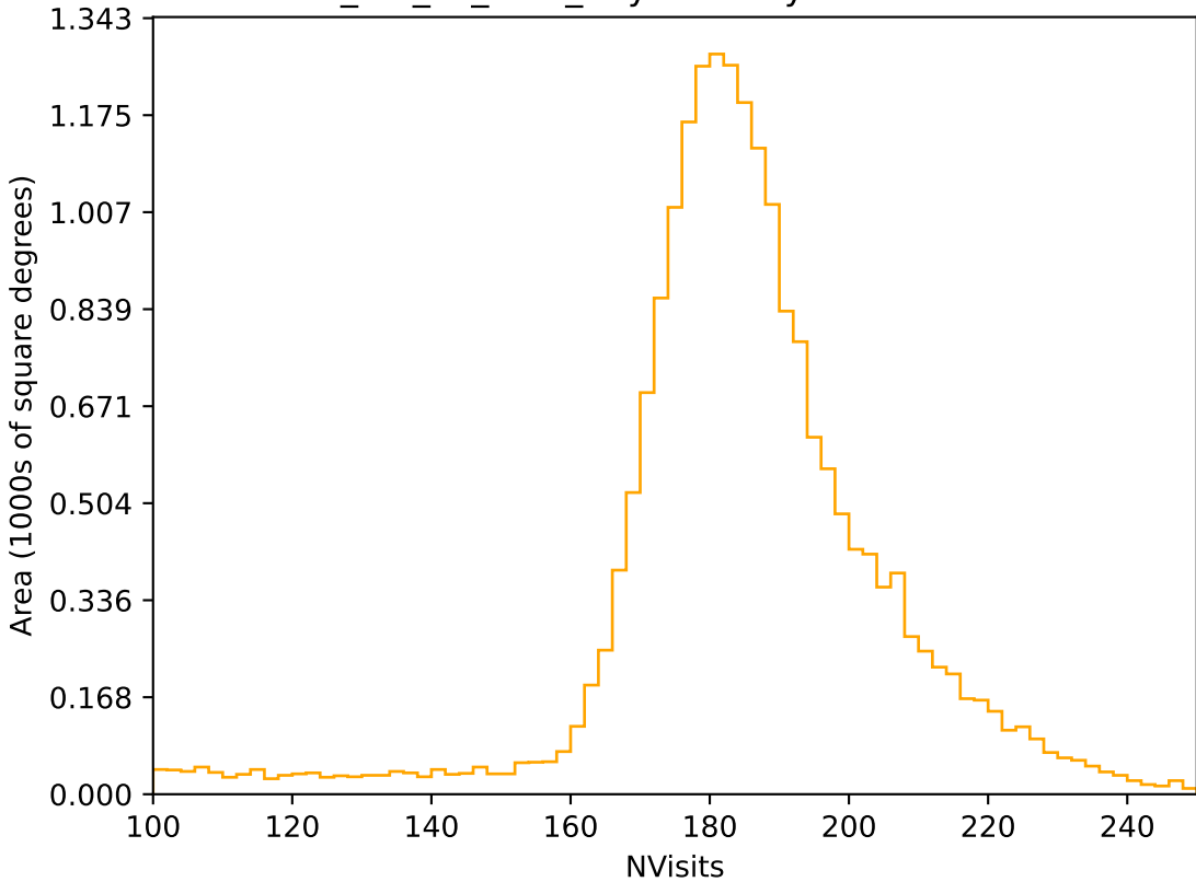
mw_roll_all_v3.3_10yrs All sky r band: NVisits
