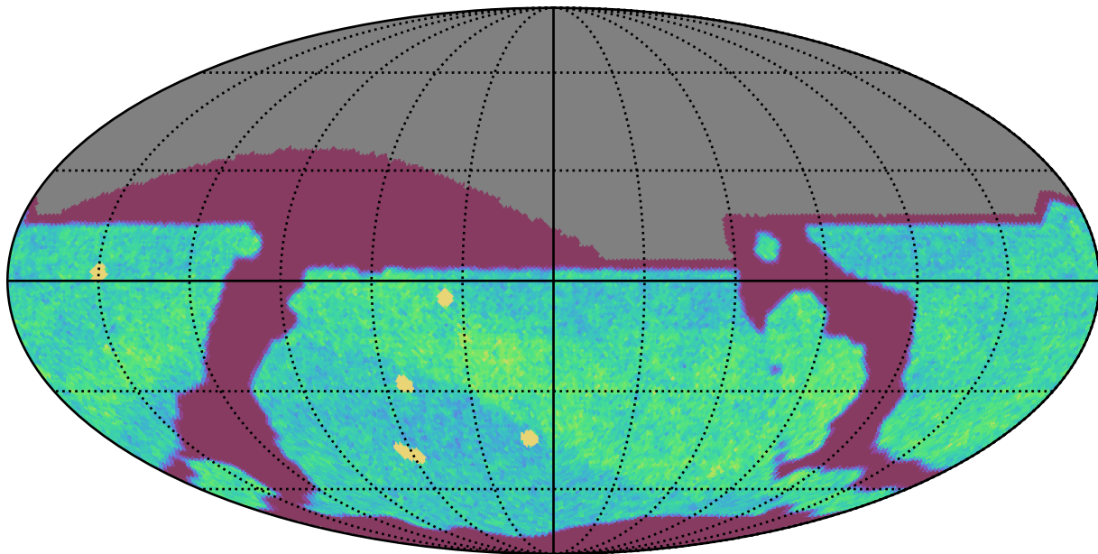
mw_roll_all_v3.3_10yrs All sky i band: NVisits
