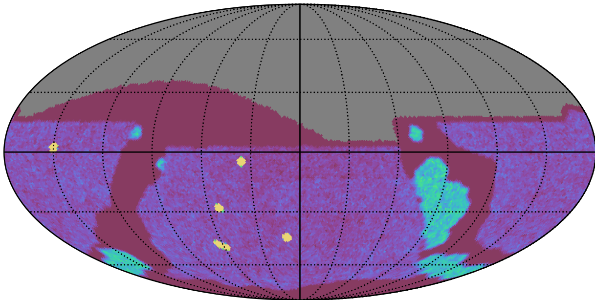
mw_roll_all_v3.3_10yrs All sky g band: NVisits
