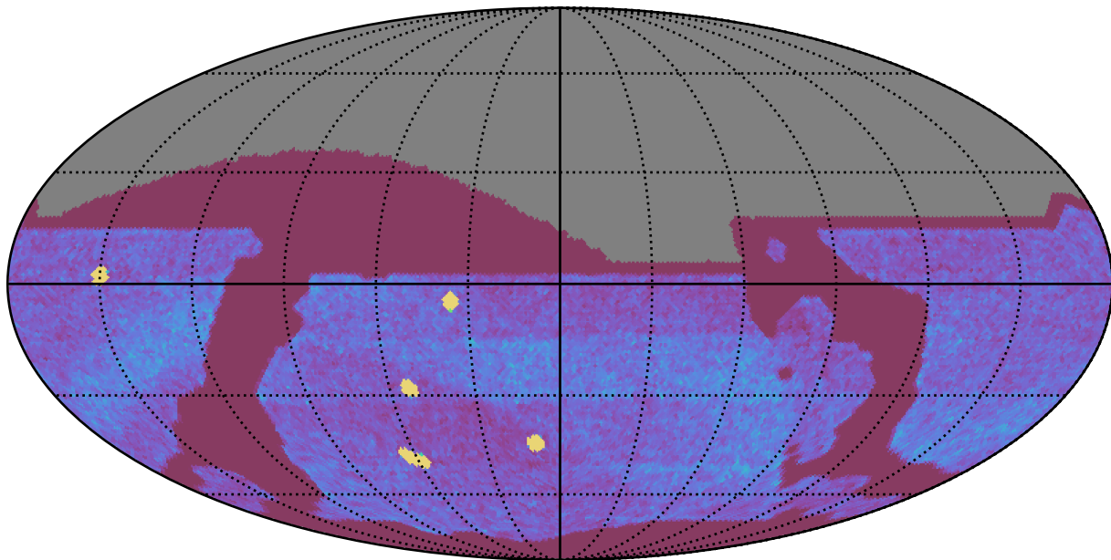
mw_roll_all_v3.3_10yrs All sky all bands: NVisits
