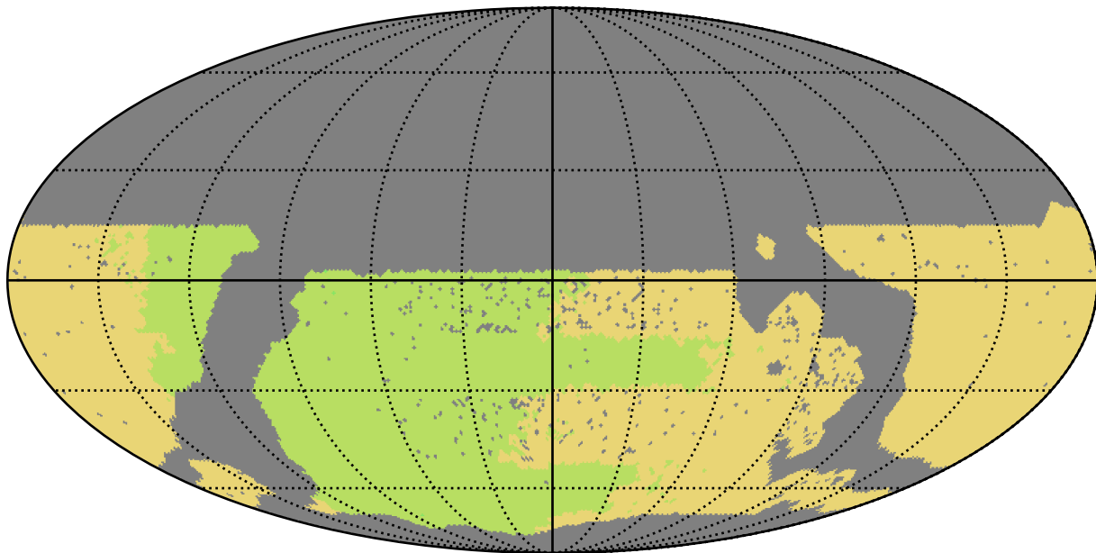
mw_roll_all_v3.3_10yrs WFD all bands: NSeasons
