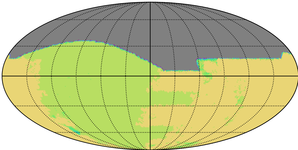
mw_roll_all_v3.3_10yrs All sky all bands: NSeasons
