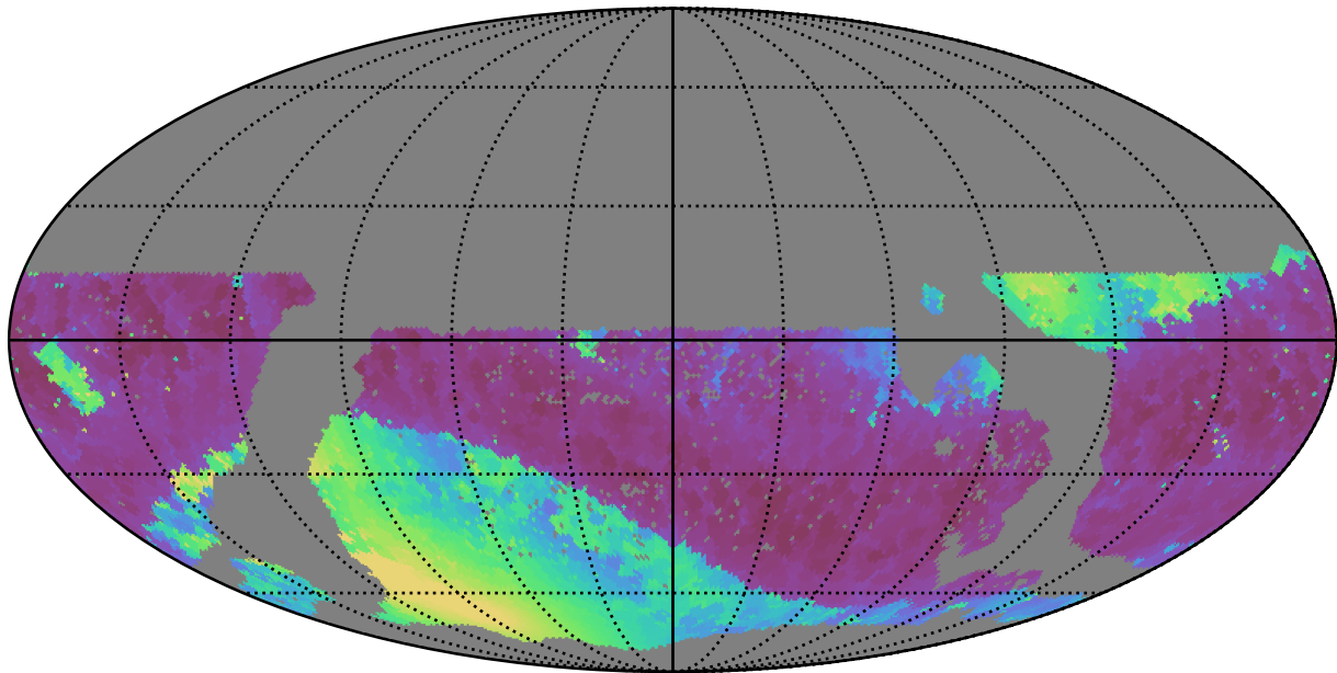
mw_roll_all_v3.3_10yrs WFD z band: Min solarElong
