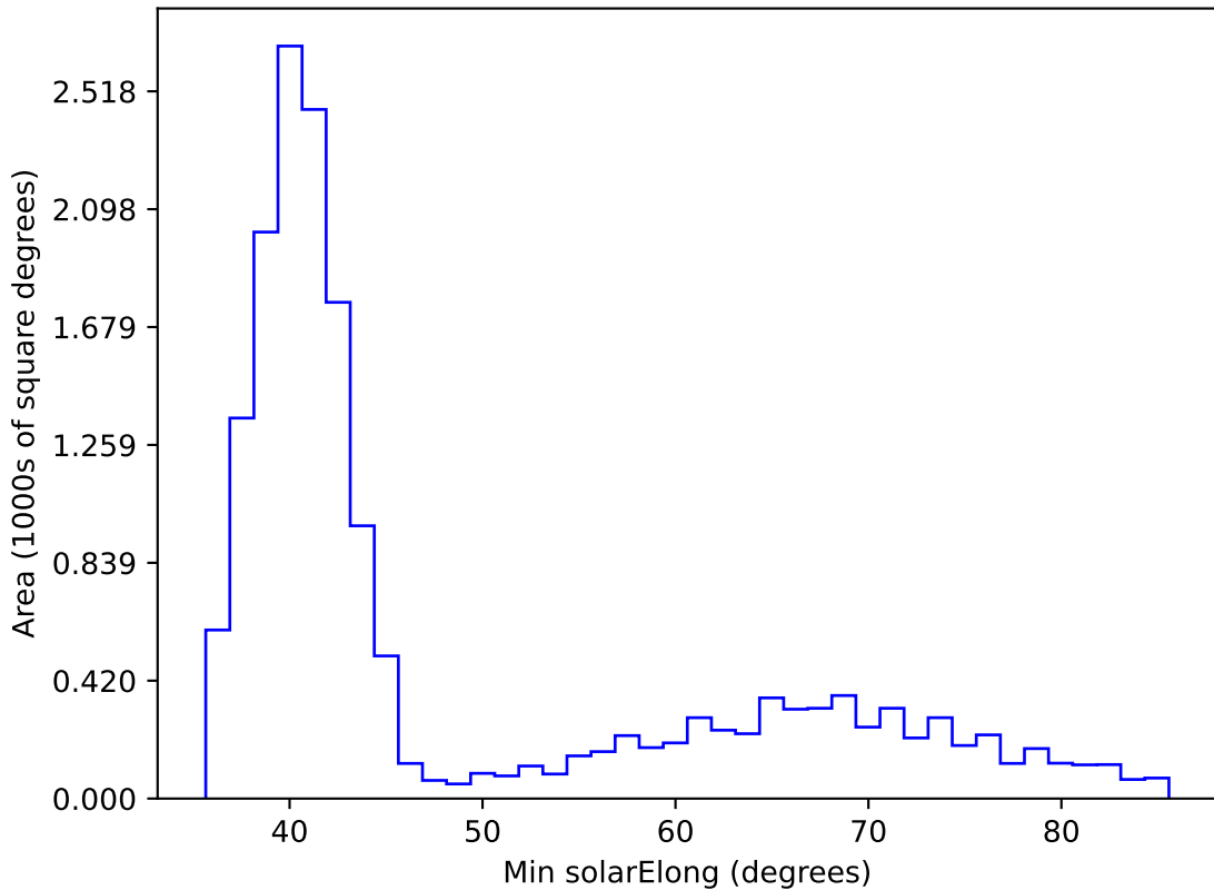
mw_roll_all_v3.3_10yrs WFD z band: Min solarElong
