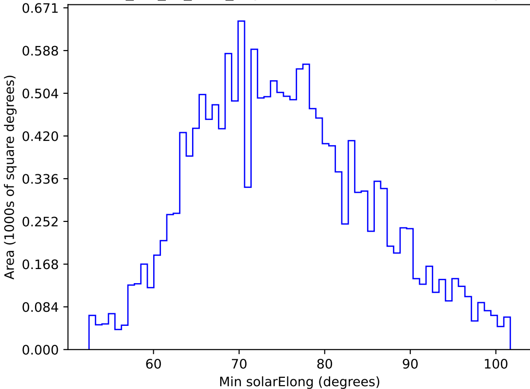
mw_roll_all_v3.3_10yrs WFD u band: Min solarElong
