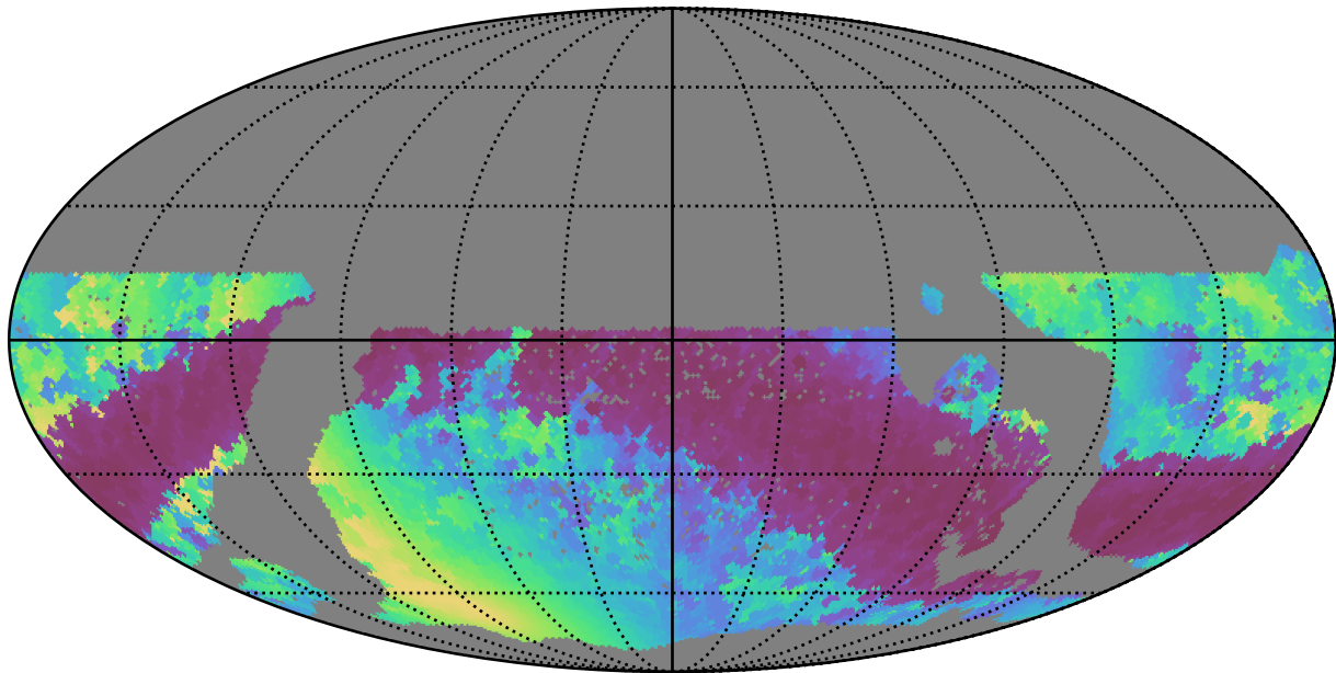
mw_roll_all_v3.3_10yrs WFD r band: Min solarElong
