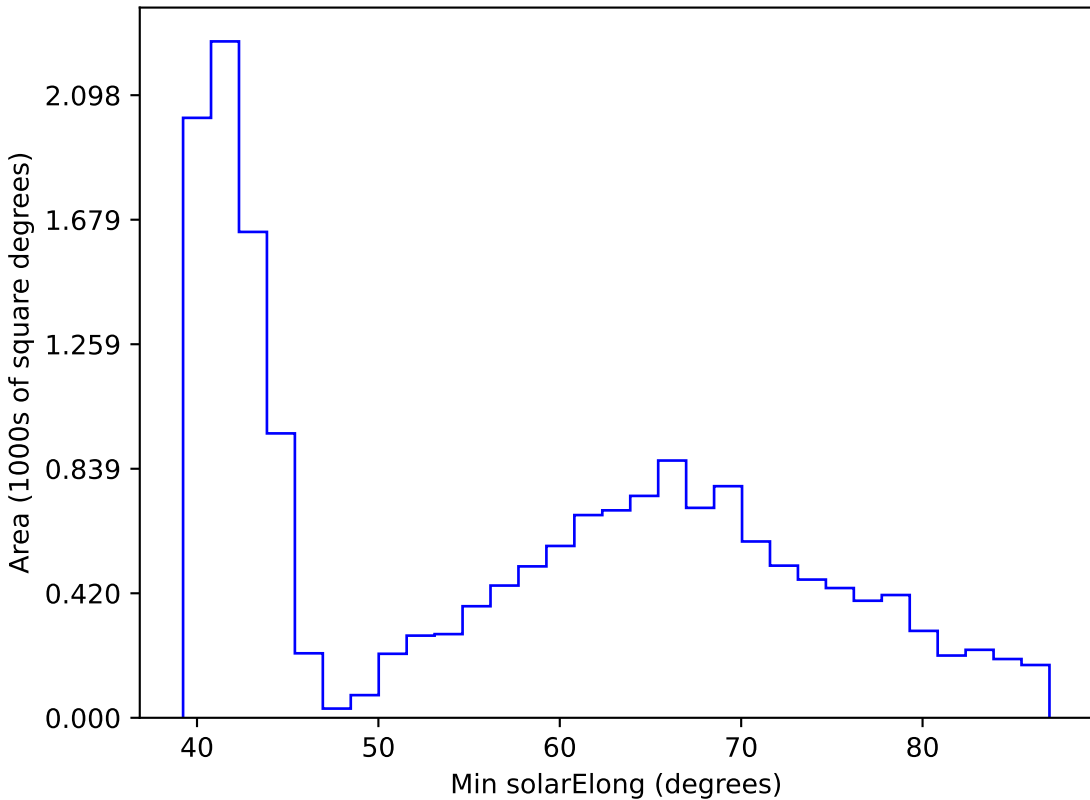
mw_roll_all_v3.3_10yrs WFD r band: Min solarElong
