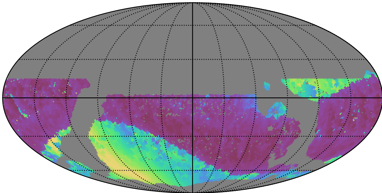
mw_roll_all_v3.3_10yrs WFD i band: Min solarElong
