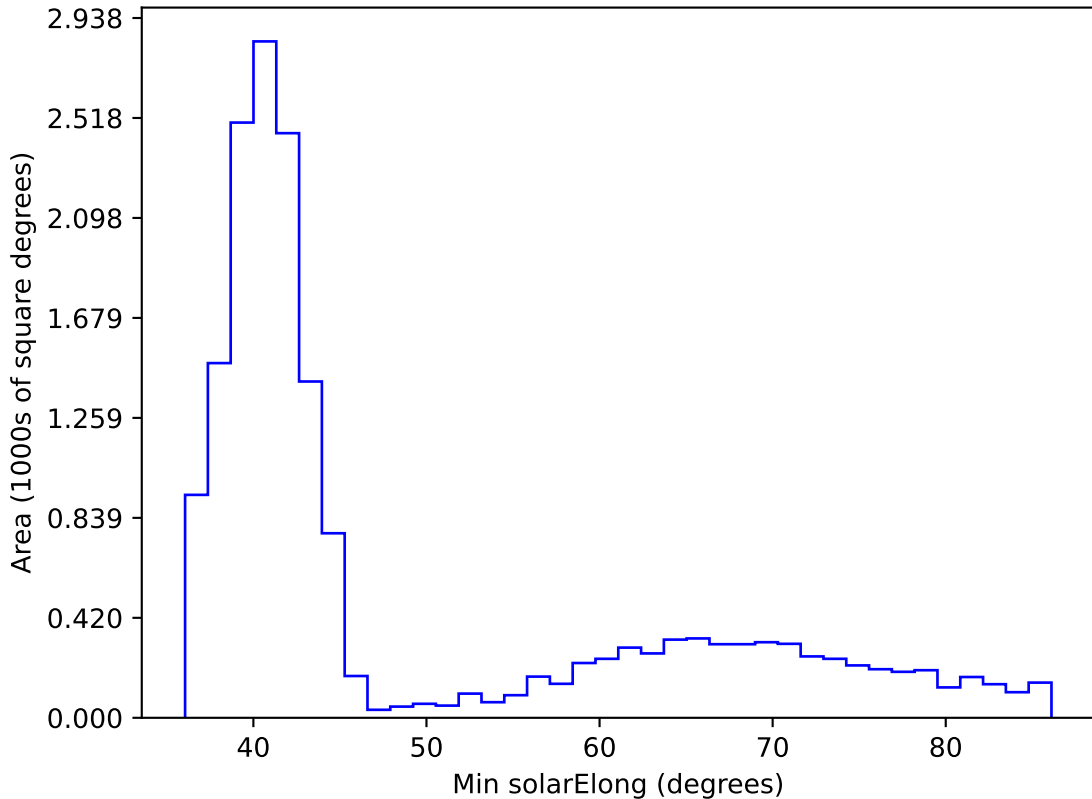
mw_roll_all_v3.3_10yrs WFD i band: Min solarElong
