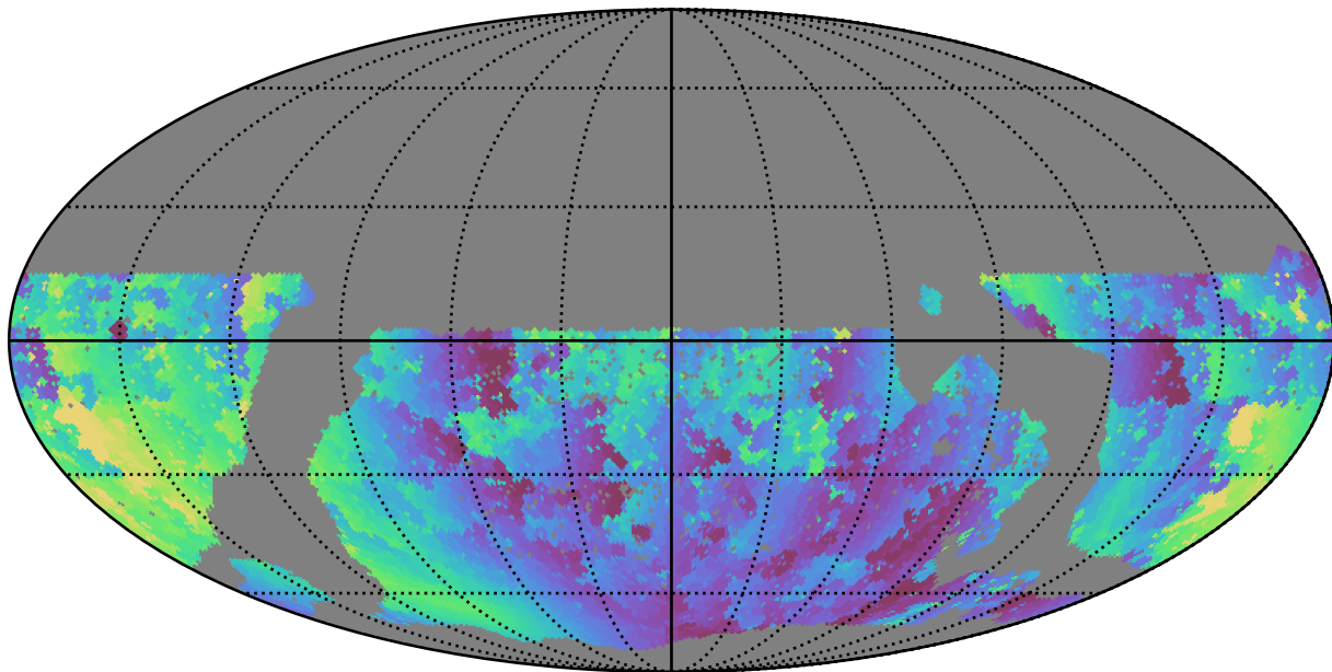
mw_roll_all_v3.3_10yrs WFD g band: Min solarElong
