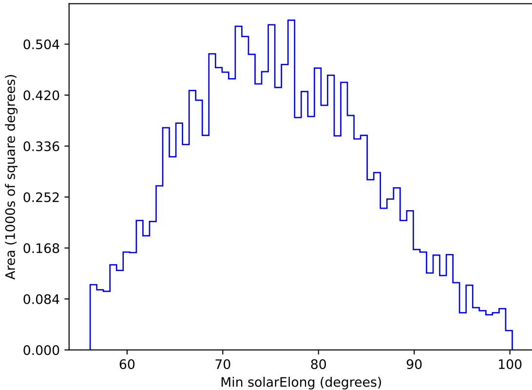
mw_roll_all_v3.3_10yrs WFD g band: Min solarElong
