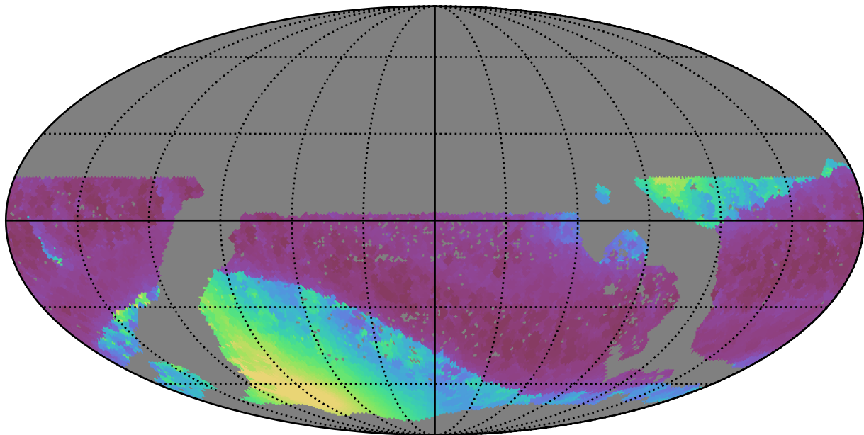
mw_roll_all_v3.3_10yrs WFD all bands: Min solarElong
