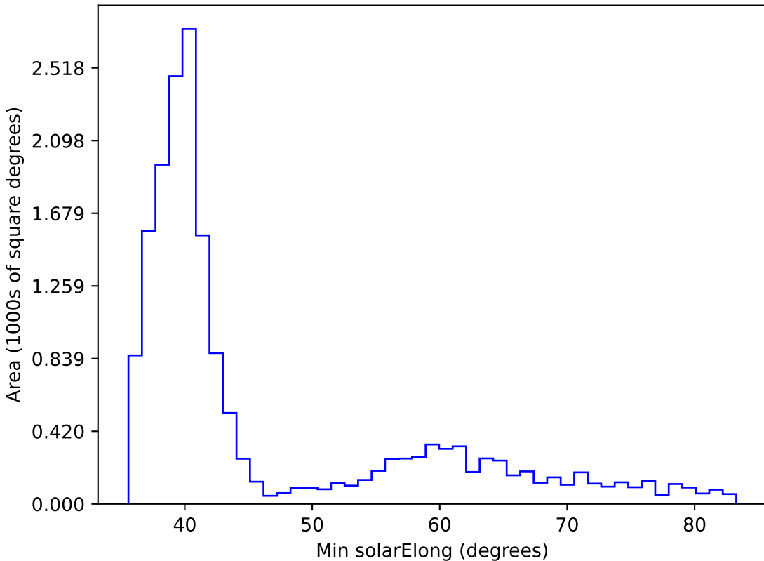
mw_roll_all_v3.3_10yrs WFD all bands: Min solarElong
