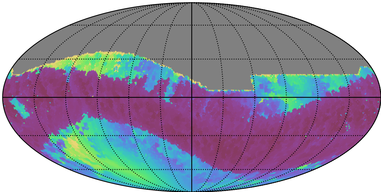
mw_roll_all_v3.3_10yrs All sky z band: Min solarElong
