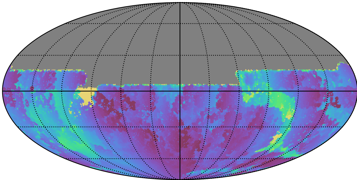
mw_roll_all_v3.3_10yrs All sky u band: Min solarElong
