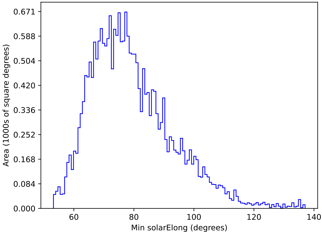
mw_roll_all_v3.3_10yrs All sky u band: Min solarElong
