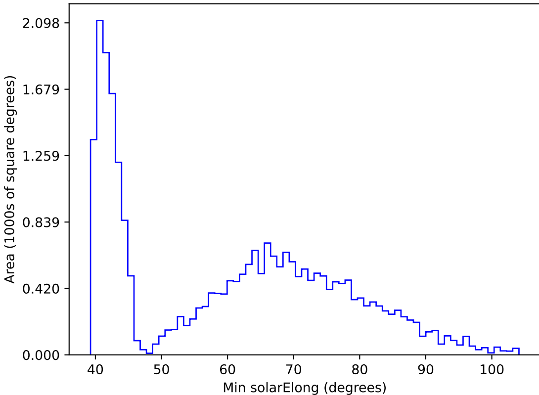
mw_roll_all_v3.3_10yrs All sky r band: Min solarElong
