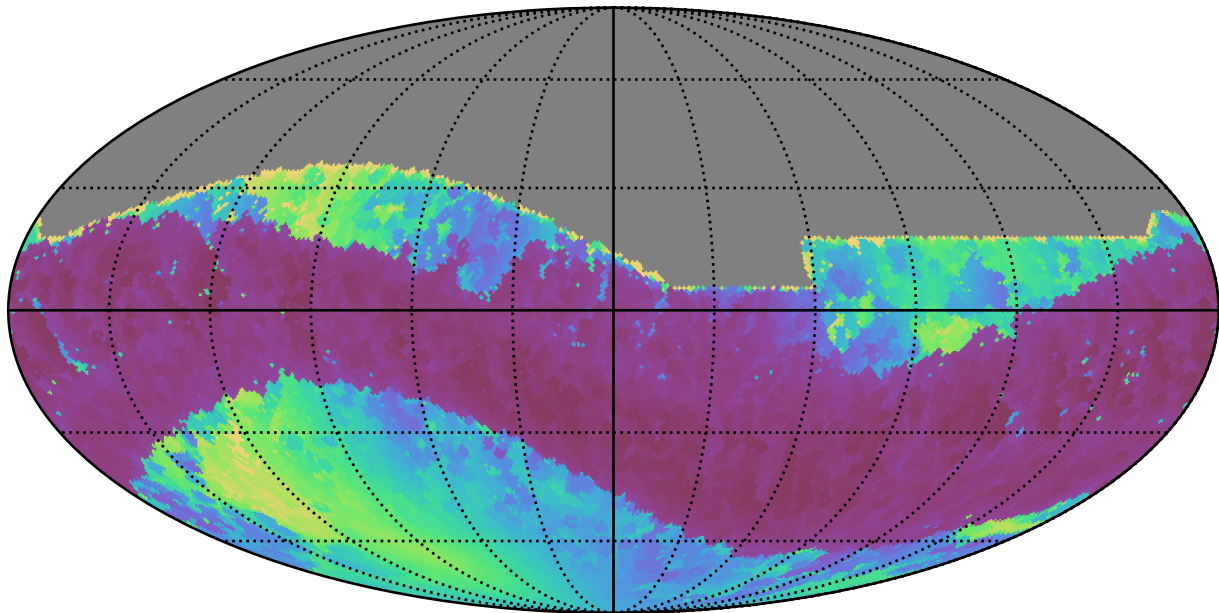
mw_roll_all_v3.3_10yrs All sky i band: Min solarElong
